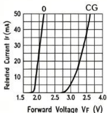
Fig.2 Forward Voltage vs. Forward Current
