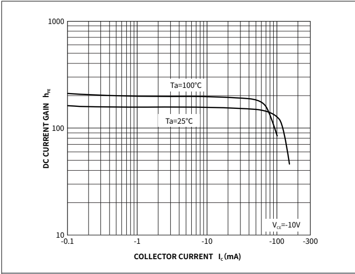
Fig.2 DC Current Gain
