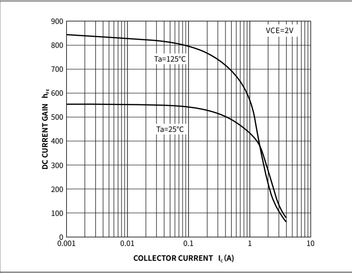
Fig.1 DC Current Gain
