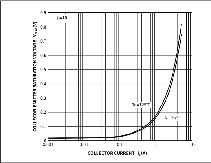
Fig.2 Collector-Emitter Saturation Voltage
