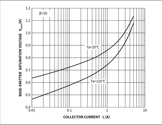
Fig.3 Base-Emitter Saturation Voltage
