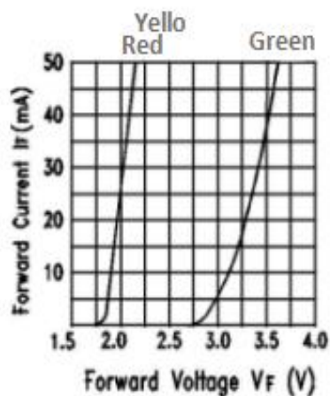
Fig.2 Forward Current vs. Forward Voltage
