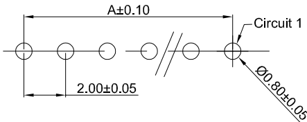
PCB REFERENCE DIAGRAM TOLERANCE:±0.05
