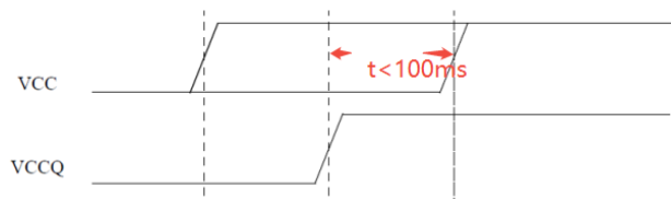
Figure.10 Schematic diagram of power-up sequence
