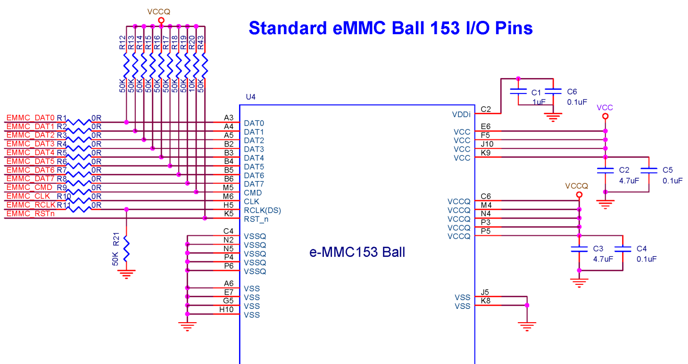
Figure.11 Schematic diagram of PCB layout
