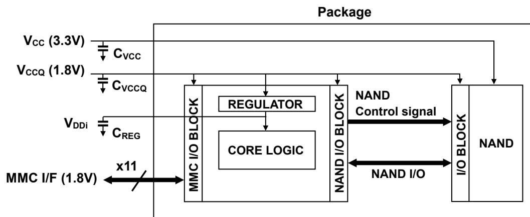
Figure 1 THGAMVG7T13BAIL Block Diagram
