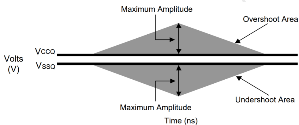
Figure.8 Overshoot/undershoot definition
