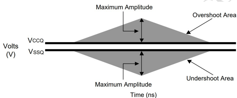
Figure.8 Overshoot/undershoot definition
