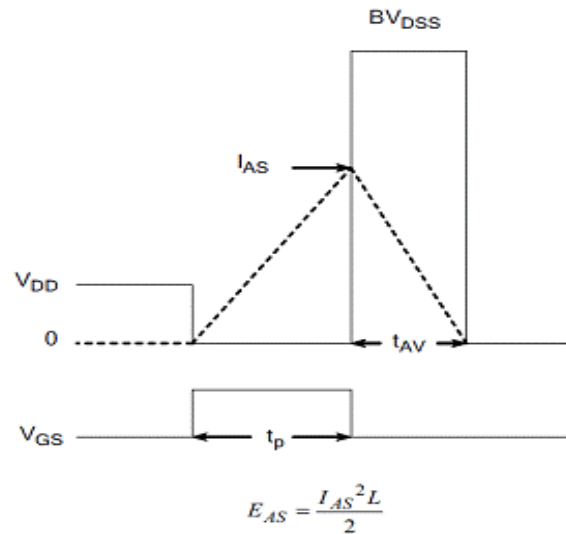
Figure21.Unclamped Inductive Switching
