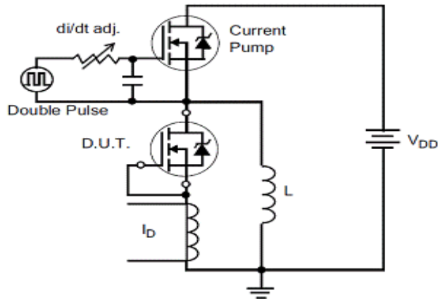
Figure 18. Diode Reverse Recovery Test Circuit Waveform
