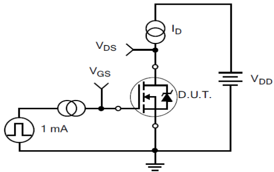
Figure 14. Gate Charge Test Circuit
