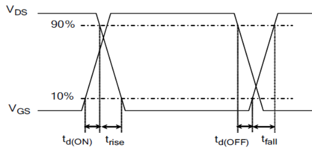
Figure 17. Resistive Switching
