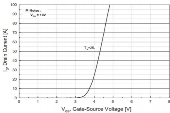
Fig.5 Transfer Characteristics
