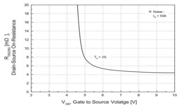
Fig.4 On-Resistance Variation with Gate to Source Voltage
