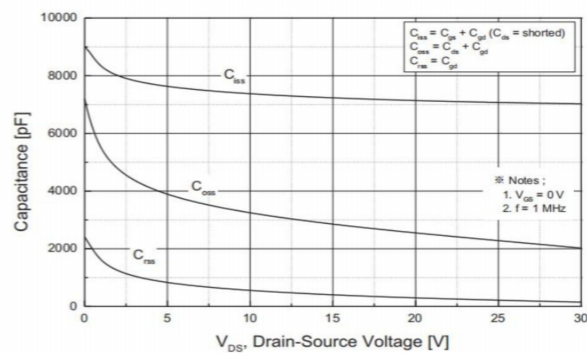
Fig.8 Capacitance Characteristics
