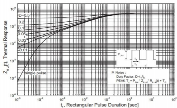
Fig.11 Transient Thermal Response Curve
