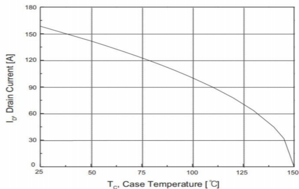
Fig.10 Maximum Drain Current vs. Case Temperature
