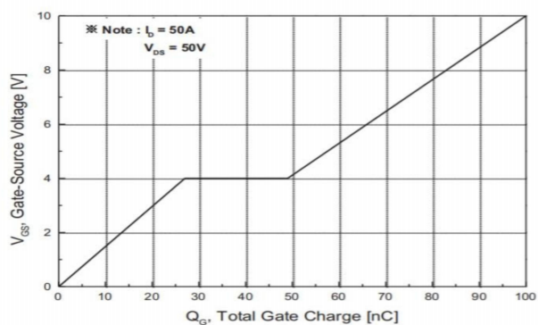
Fig.7 Gate Charge Characteristics
