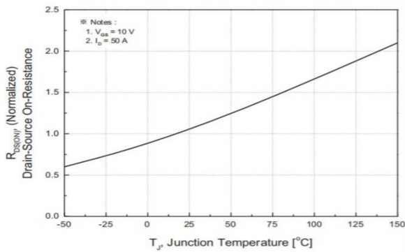
Fig.3 On-Resistance Variation with Temperature
