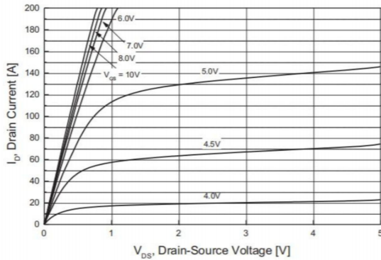
Fig.1 On-Region Characteristics
