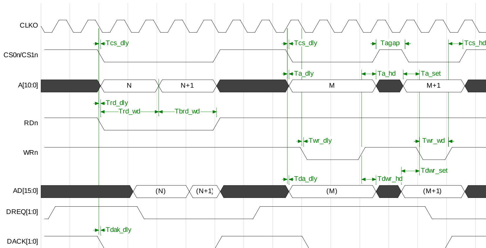
Figure 4-5: Non-multiplexed Bus Type with Internal Cycle Count Timing Diagram
