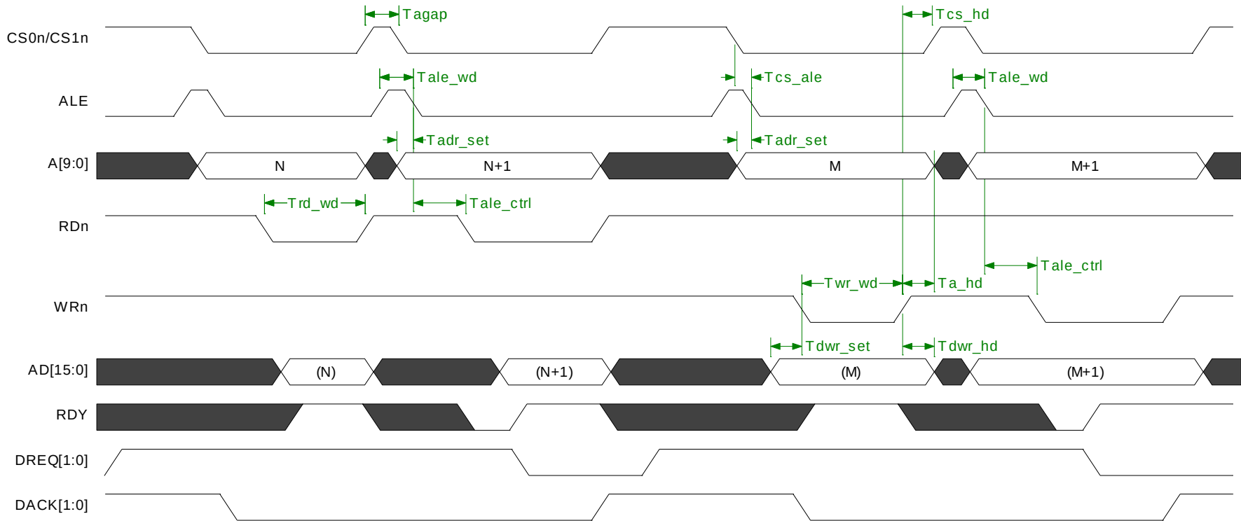
Figure 4-9: ISA-Like Bus Type with External RDY Timing Diagram
