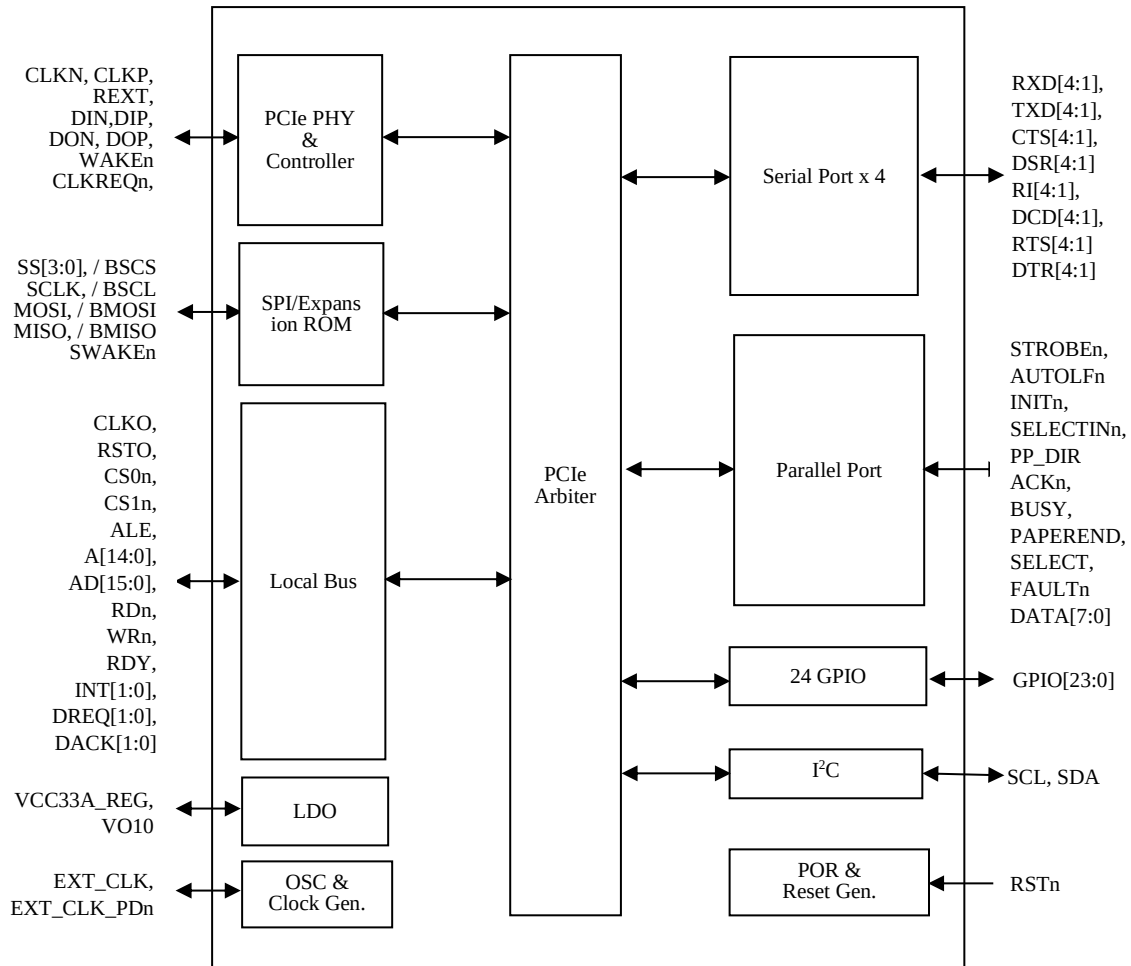
Figure 1-1: AX99100A Block Diagram
