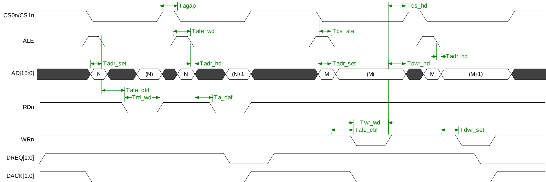
Figure 4-12: Non-multiplexed Bus Type with Internal Cycle Count Timing Diagram
