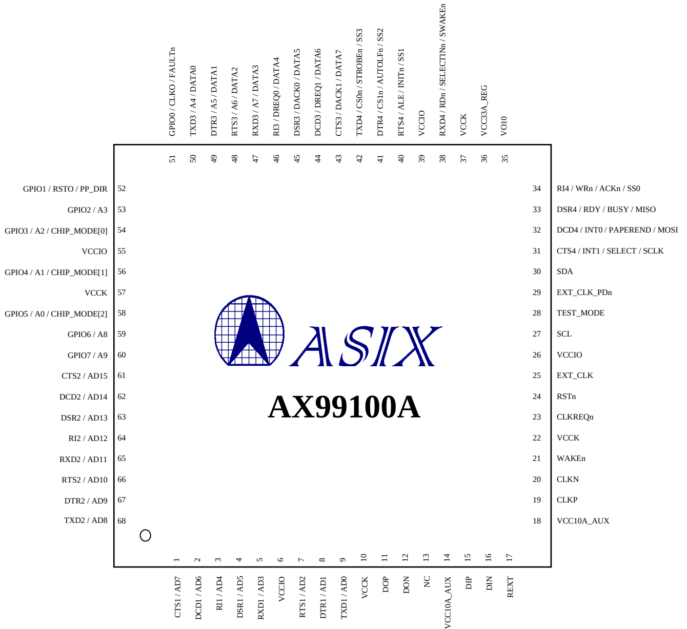
Figure 1-2: AX99100A Pinout Diagram
