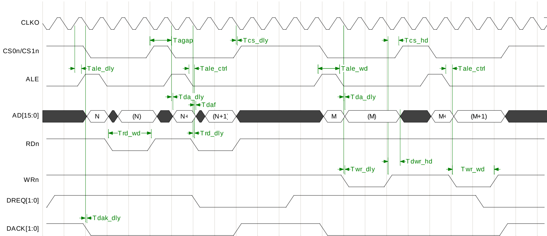
Figure 4-7: Multiplexed Bus Type with Internal Cycle Count Timing Diagram
