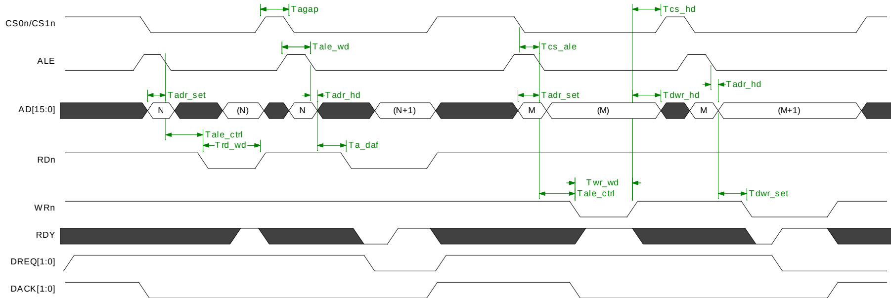
Figure 4-11: Multiplexed Bus Type with External RDY Timing Diagram
