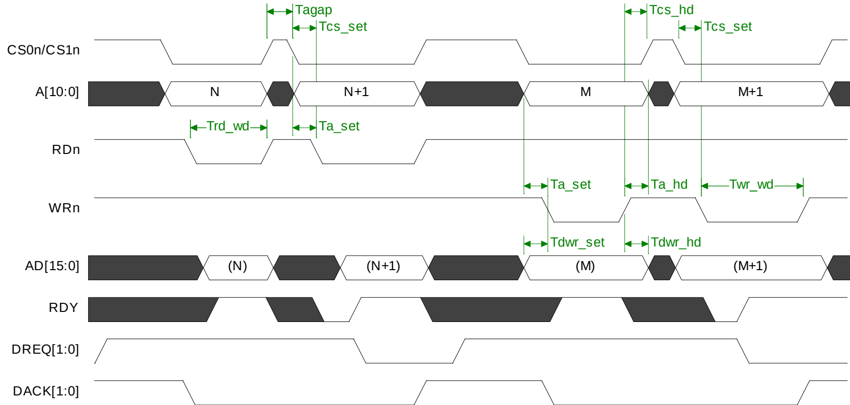
Figure 4-8: Non-multiplexed Bus Type with External RDY Timing Diagram
