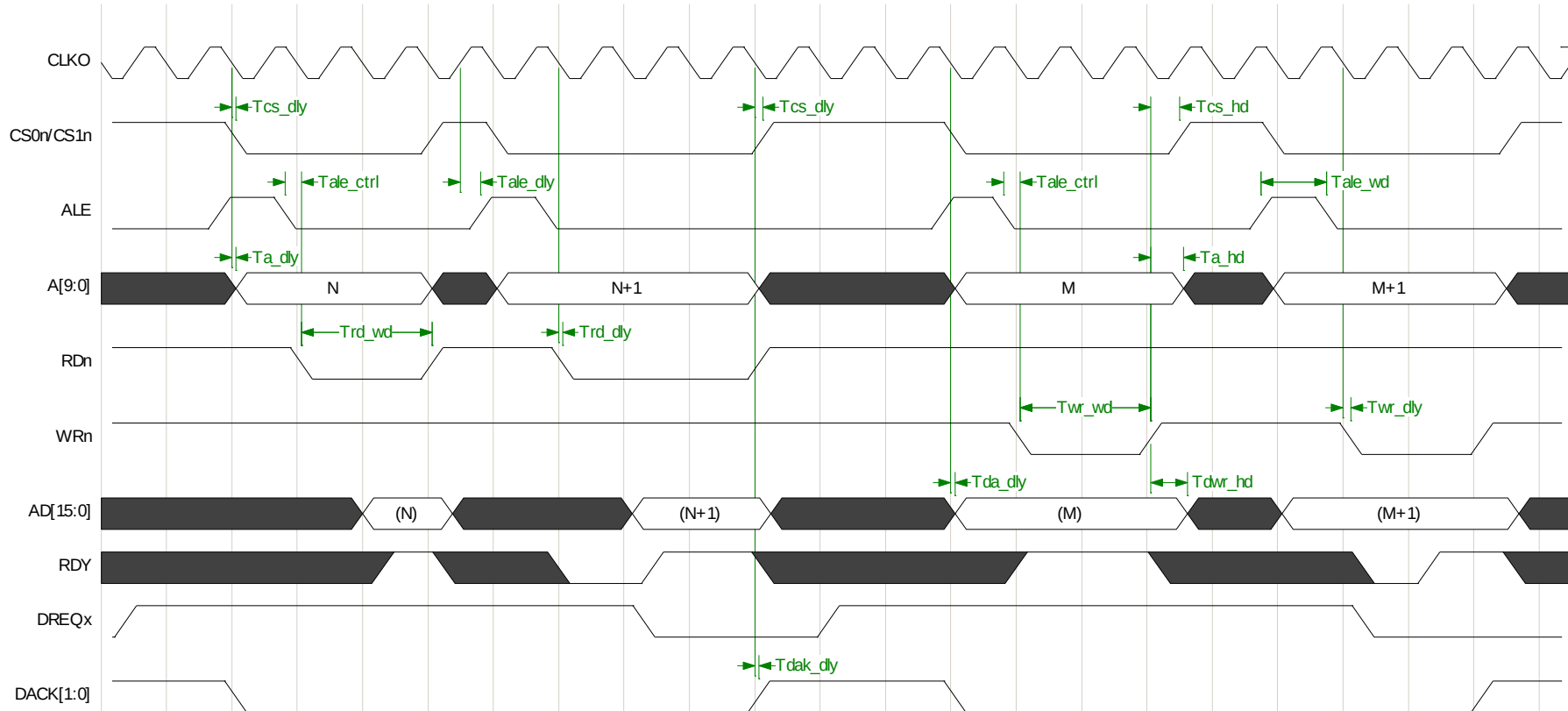
Figure 4-4: ISA-Like Bus Type with External RDY Timing Diagram
