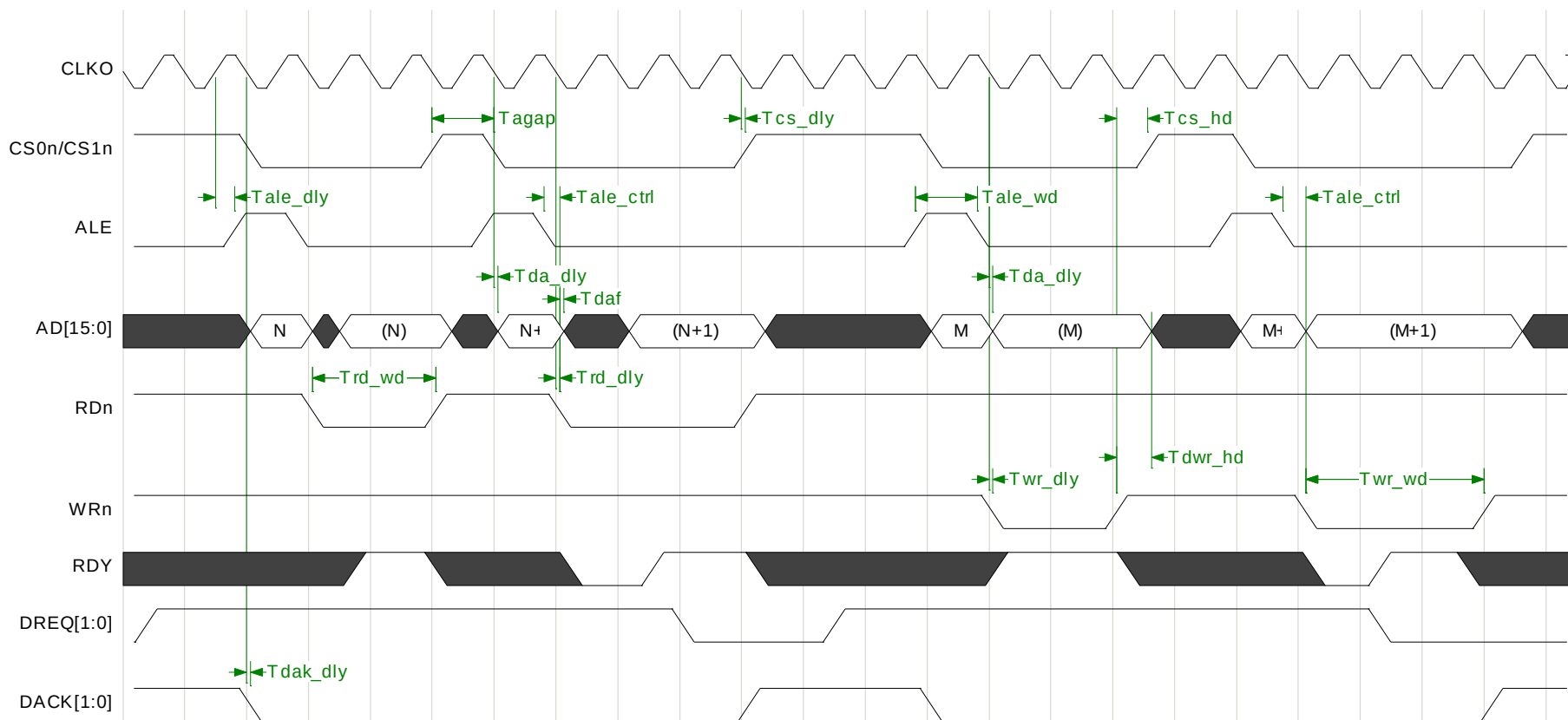
Figure 4-6: Multiplexed Bus Type with External RDY Timing Diagram
