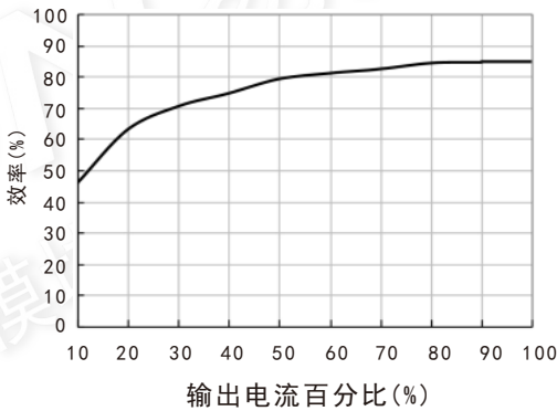
效率Vs输出负载(Vin=24V) WRE2415S-3WR2
