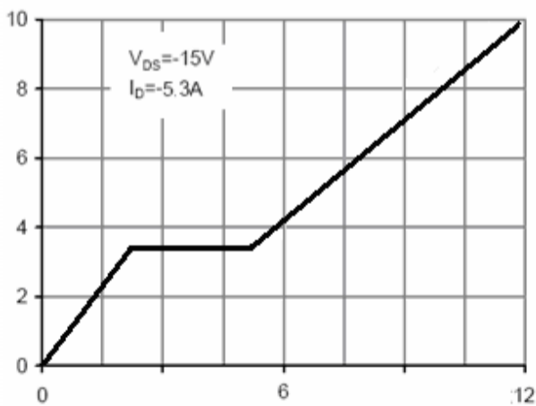
Q g Gate Charge (nC) Figure 11 Gate Charge
