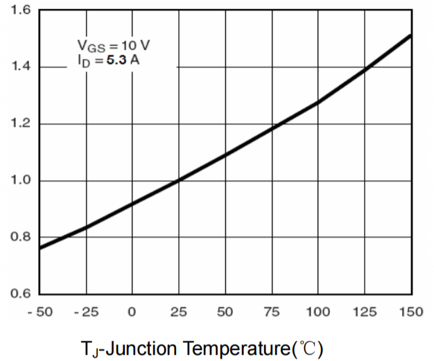
T_J -Junction Temperature( ^\circ C ) Figure 8 Drain-Source On-Resistance
