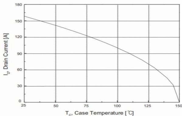
Fig.10 Maximum Drain Current vs. Case Temperature
