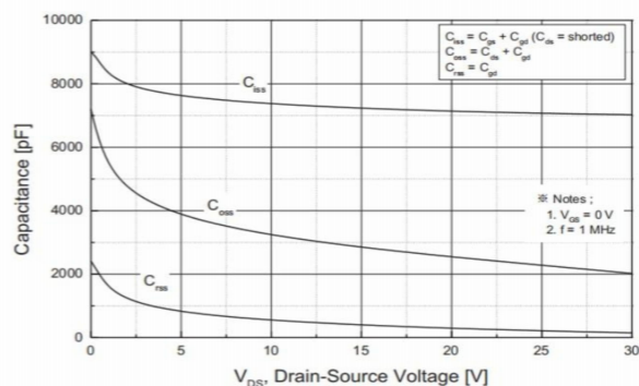
Fig.8 Capacitance Characteristics
