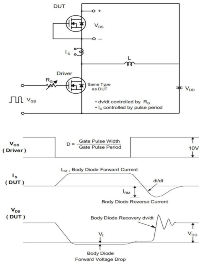
Fig 15. Peak Diode Recovery dv/dt Test Circuit & Waveforms
