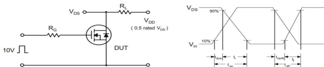
Fig 13. Resistive Switching Test Circuit & Waveforms
