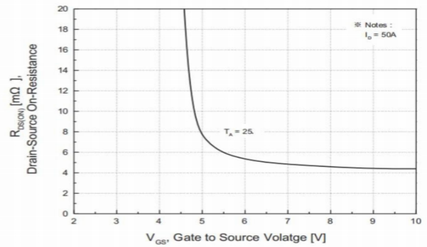
Fig.4 On-Resistance Variation with Gate to Source Voltage
