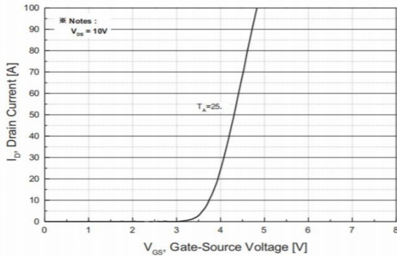
Fig.5 Transfer Characteristics
