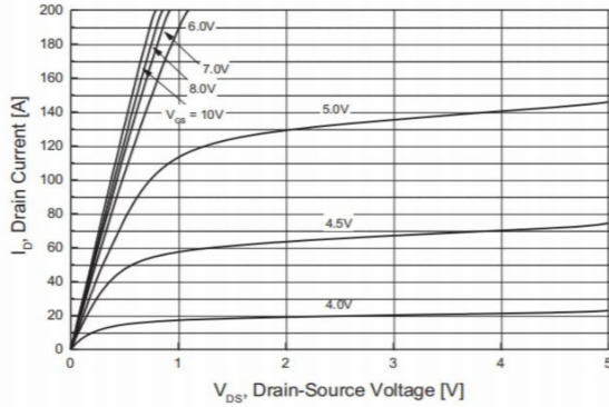
Fig.1 On-Region Characteristics
