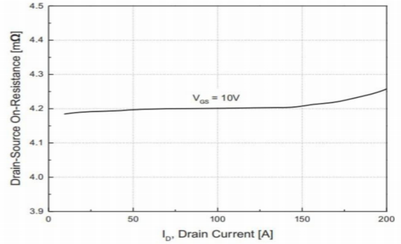
Fig.2 On-Resistance Variation with Drain Current and Gate Voltage
