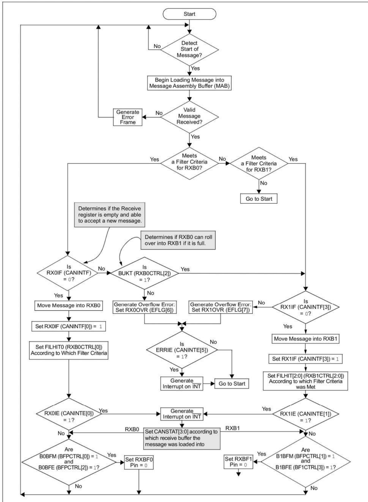
FIGURE 4-3: RECEIVE FLOWCHART
