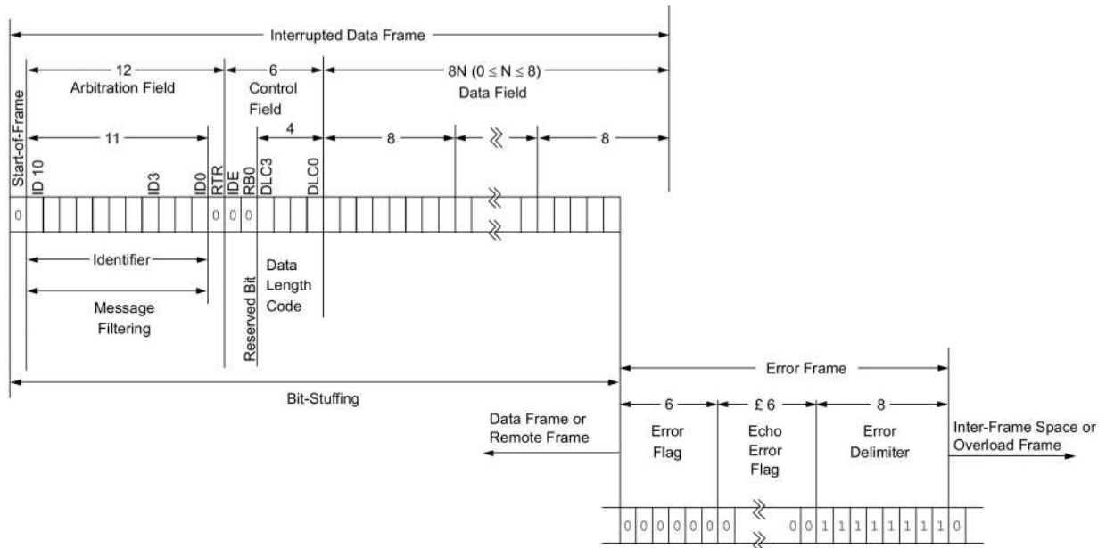
FIGURE 2-4: ACTIVE ERROR FRAME
