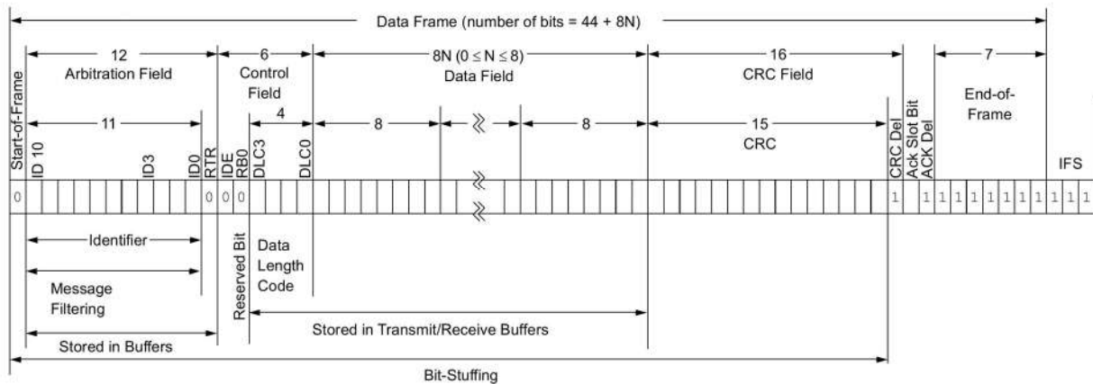
FIGURE 2-1: STANDARD DATA FRAME
