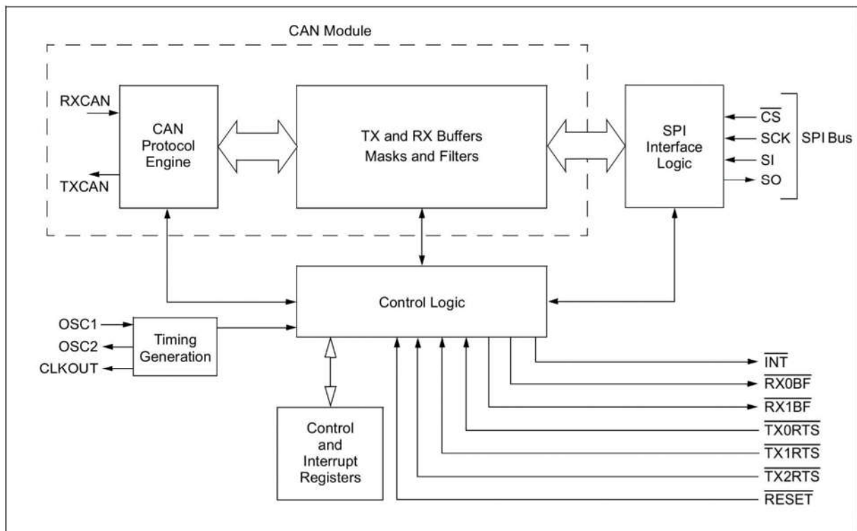
Figure 1-1 BLOCK DIAGRAM
