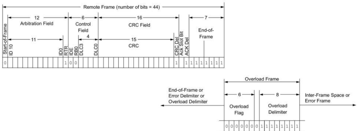
FIGURE 2-5: OVERLOAD FRAME
