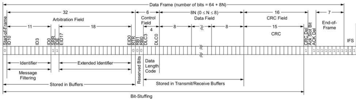
FIGURE 2-2: EXTENDED DATA FRAME
