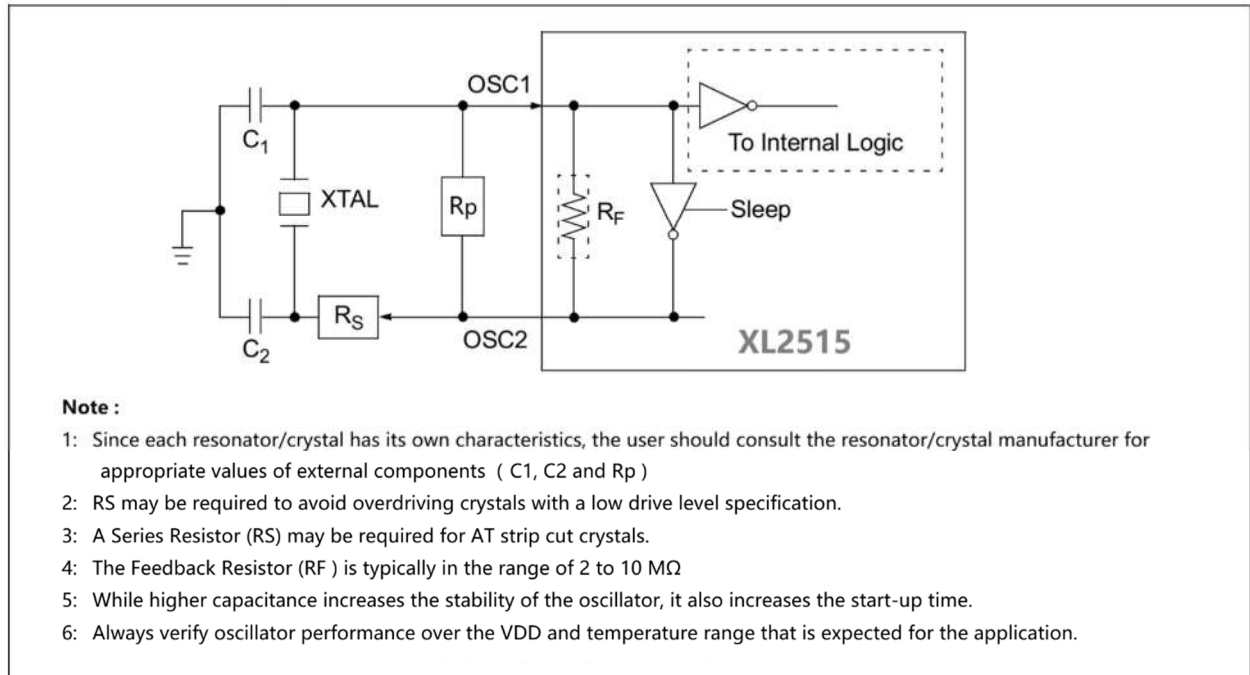
FIGURE 8-1: CRYSTAL/CERAMIC RESONATOR OPERATION
