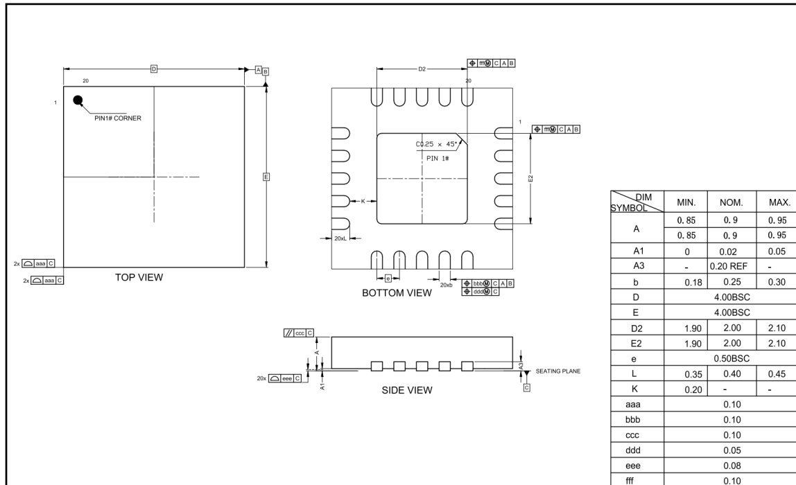
FIGURE 17 : QFN20 Package dimensions
