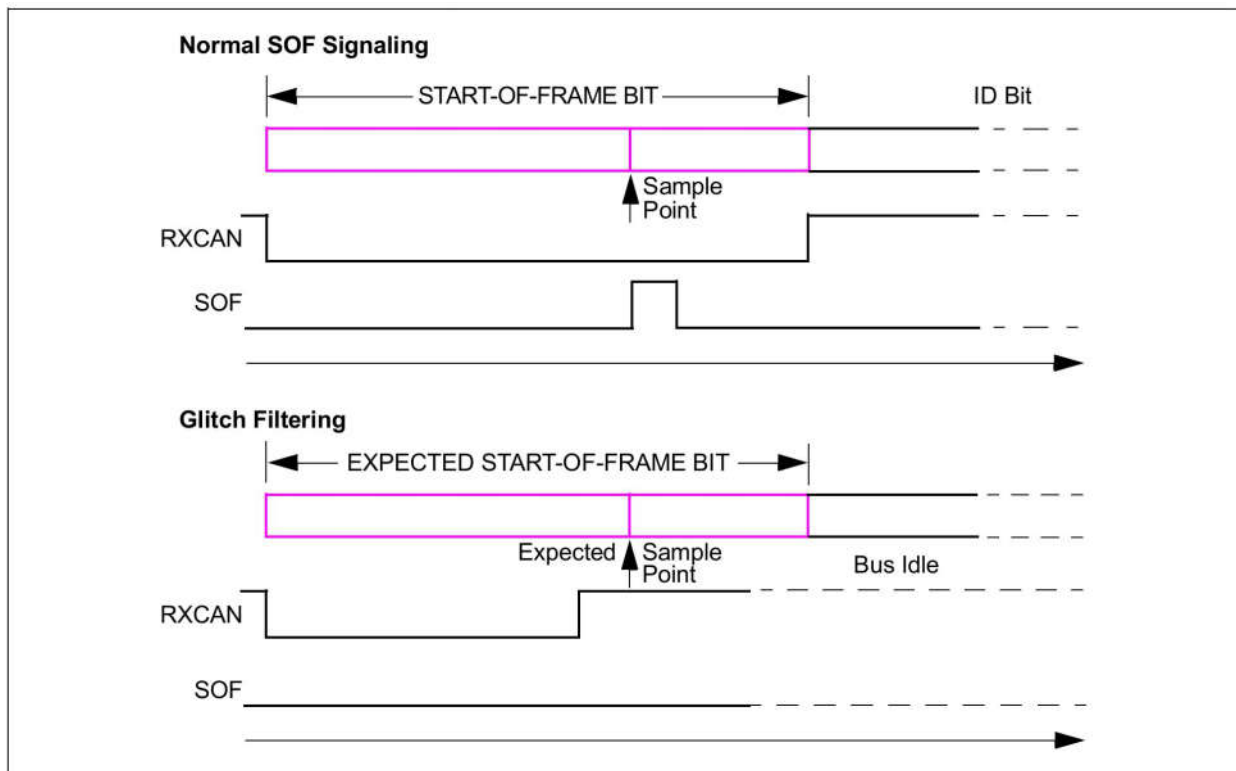
FIGURE 4-1: START-OF-FRAME SIGNALING
