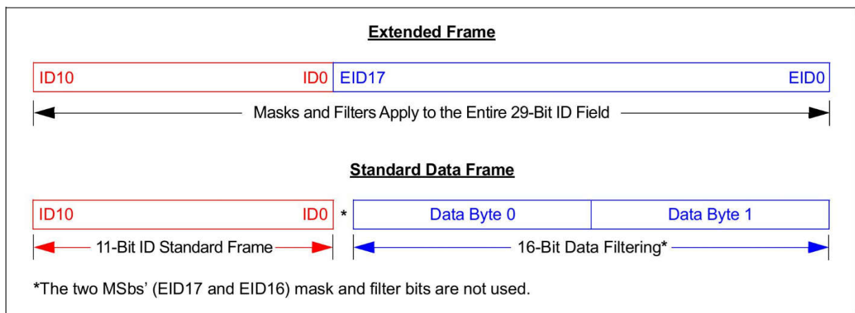
FIGURE 4-4: MASKS AND FILTERS APPLY TO CAN FRAMES
