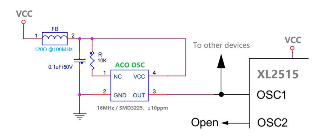
FIGURE 8-3: USING ACO (ACTIVE CRYSTAL OSCILLATOR) AS THE CLOCK SOURCE
