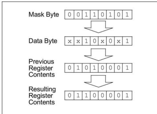
FIGURE 12-1: BIT MODIFY
