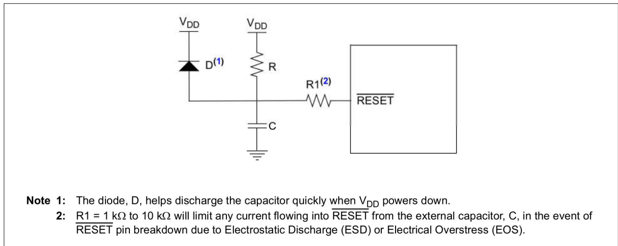
FIGURE 9-1: RESET PIN CONFIGURATION EXAMPLE
