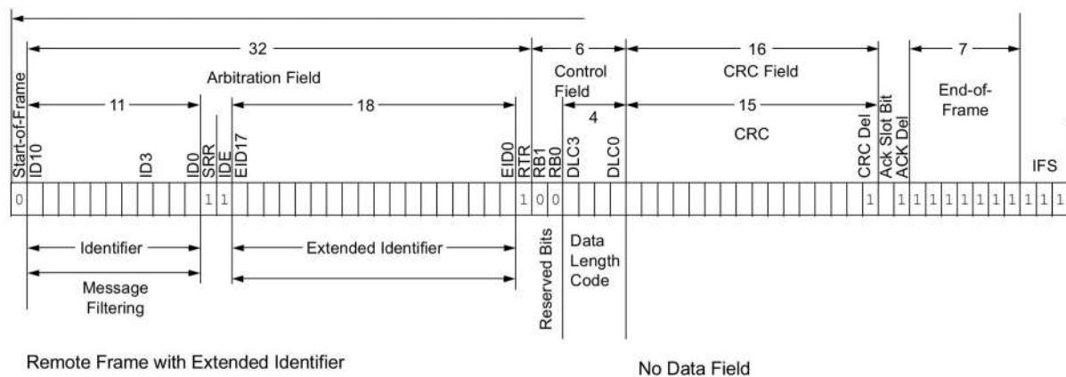
FIGURE 2-3: REMOTE FRAME
