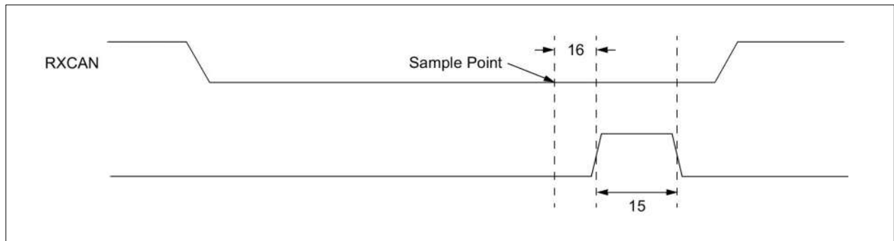
FIGURE 13-1: START-OF-FRAME PIN AC CHARACTERISTICS
