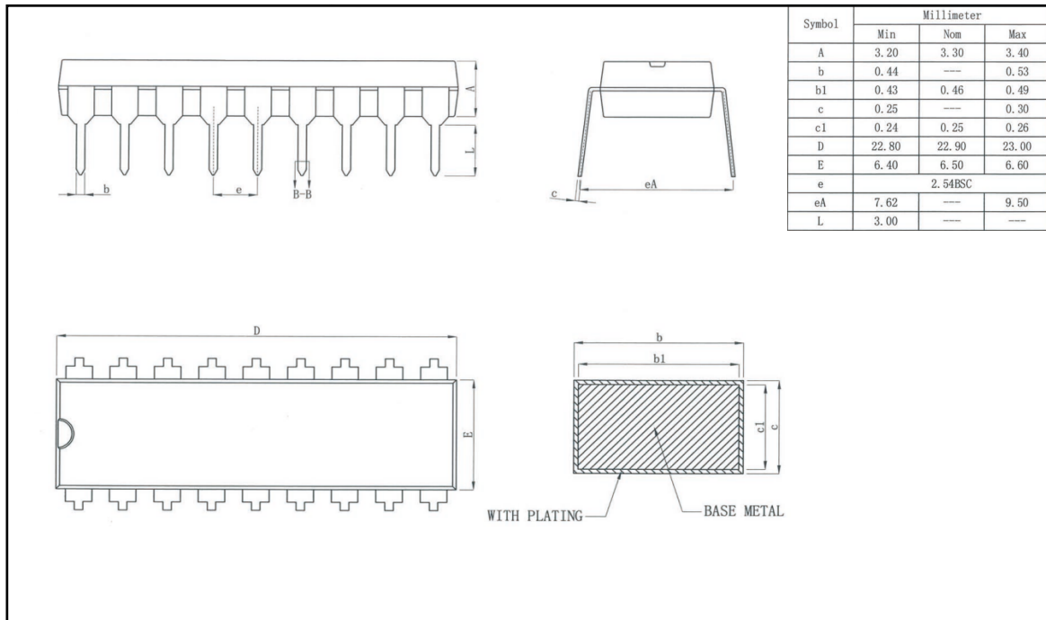
FIGURE 15 : DIP18 Package dimensions
