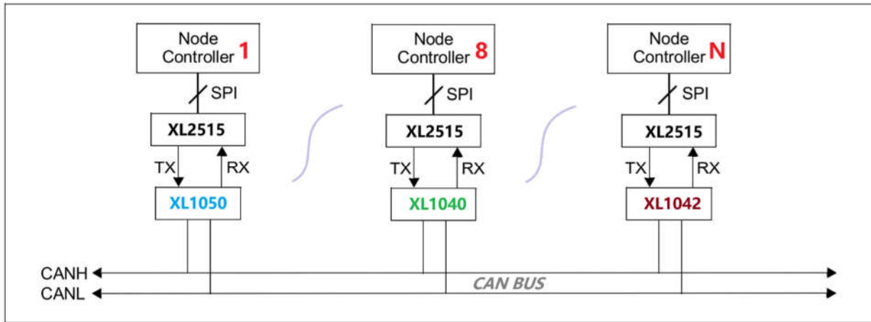
Figure 1-2 EXAMPLE SYSTEM IMPLEMENTATION FOR CAN BUS
