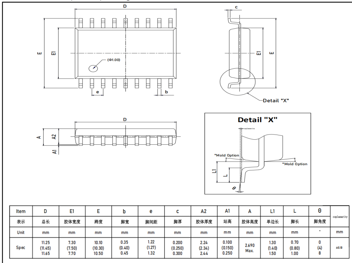
FIGURE 14 : SOP18 ( 300mil ) Package outline dimensions
