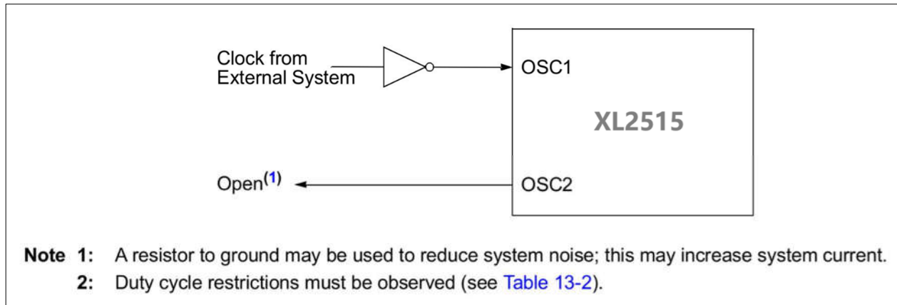
FIGURE 8-2: EXTERNAL CLOCK SOURCE
