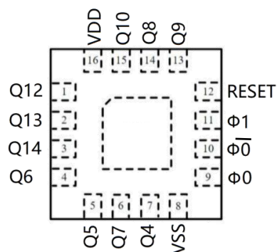
QFN-16 3*3
