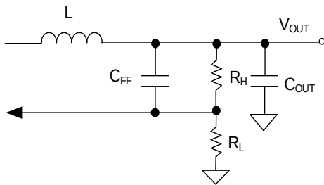
Figure7. Feedforward Network
