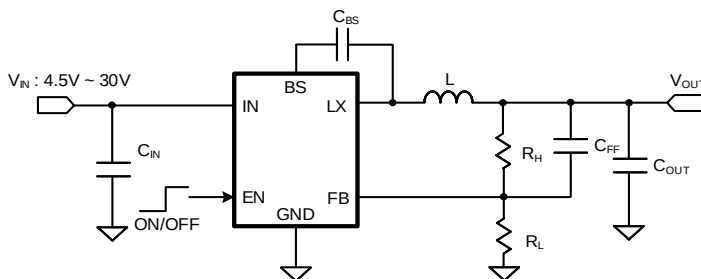
Figure1. Schematic Diagram
