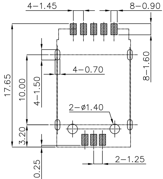
PCB Layout Diagram Top View
