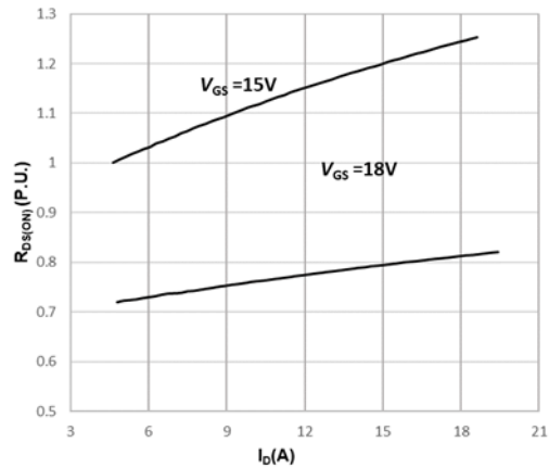
Fig6. Normalized On-Resistance vs. Drain Current For
