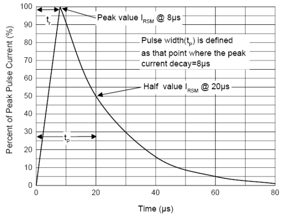
8 X 20 \mu s Pulse Waveform
