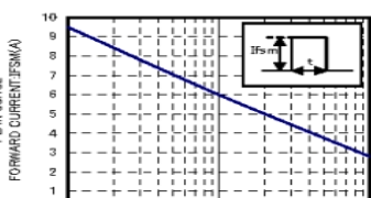
IFSM-t CHARACTERISTICS
