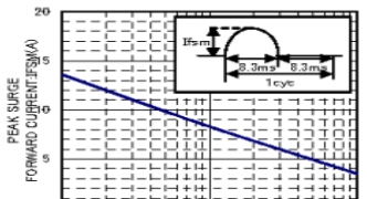
IFSM-CYCLE CHARACTERISTICS
