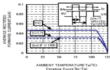
AMBIENT TEMPERATURE (Ta) (°C) Derating Curve (IA-Ta)
