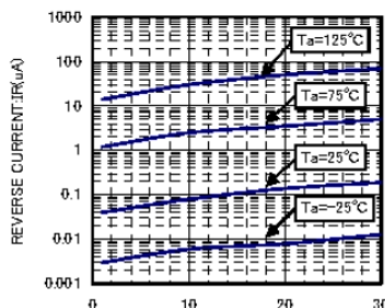
VR-IR CHARACTERISTICS
