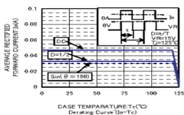
CASE TEMPERATURE (Tc) (°C) Derating Curve (IA-Tc)
