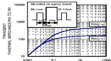
Rth-t CHARACTERISTICS
