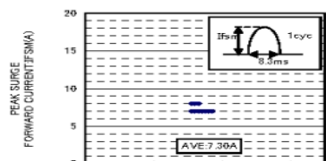
IFSM DISPERSION MAP
