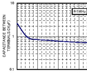
VR-Ct CHARACTERISTICS
