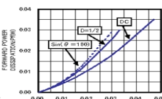
AVERAGE RECTIFIED FORWARD CURRENT (IA) IA-PF CHARACTERISTICS
