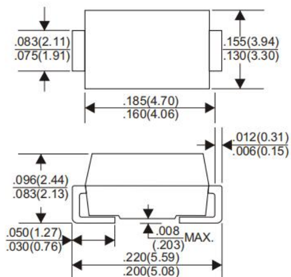
DO-214AA(SMB)
