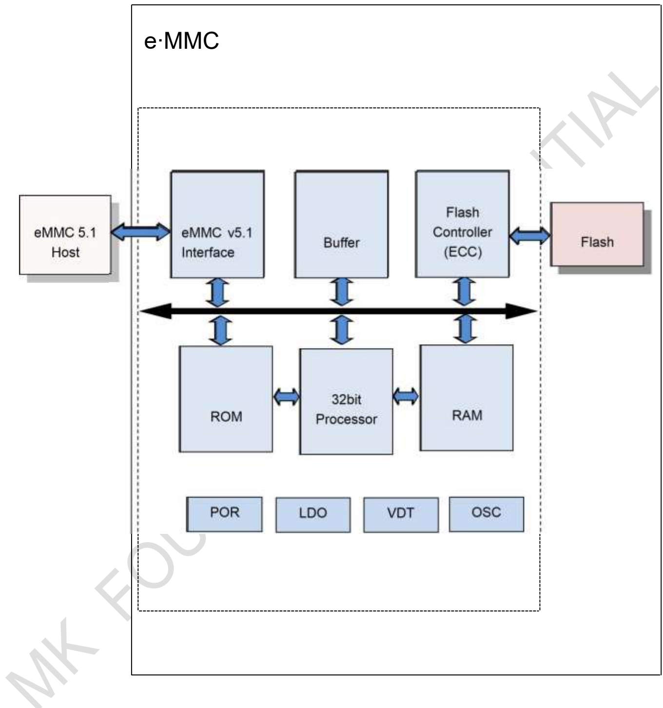
Figure 1 - eMMC Block Diagram
