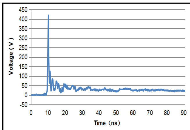
Figure 2: ESD Waveform after Clamping
