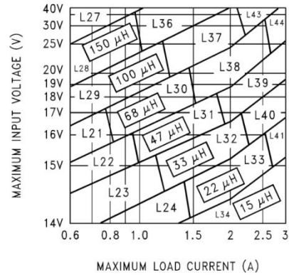
FIGURE 6. XH2596-12
