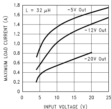
FIGURE 26. Inverting Regulator Typical Load Current
