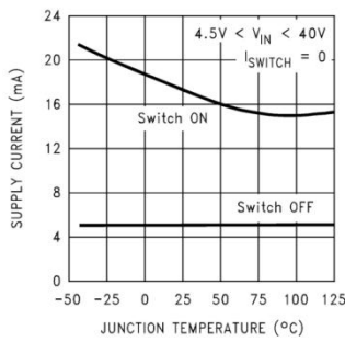
Operating Quiescent Current
