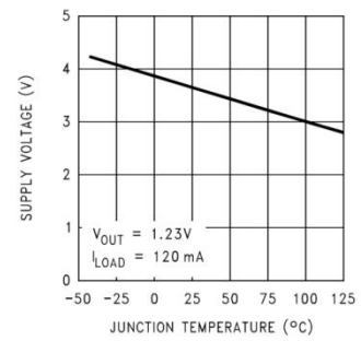
Minimum Operating Supply Voltage
