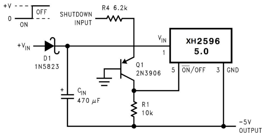
FIGURE 27. Inverting Regulator Ground Referenced Shutdown
