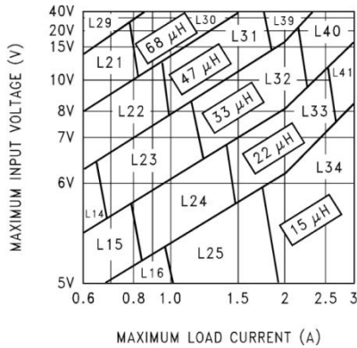
FIGURE 4. XH2596-3.3
