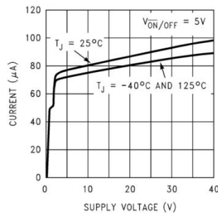
Shutdown Quiescent Current
