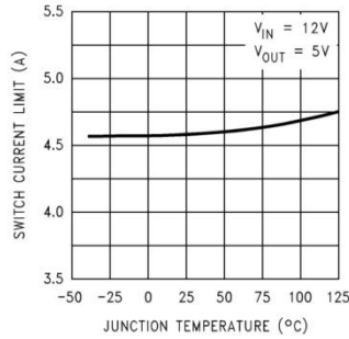
Switch Current Limit
