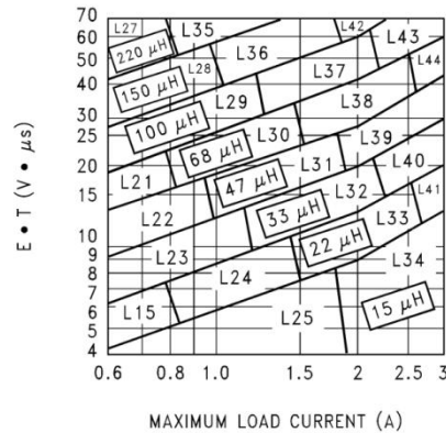
FIGURE 7. XH2596-ADJ
