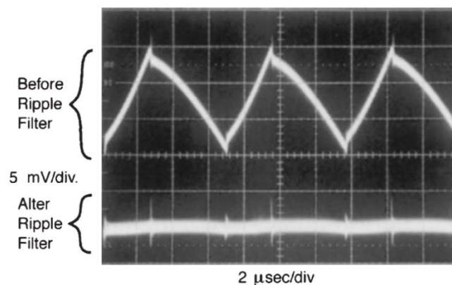
FIGURE 17. Post Ripple Filter Waveform
