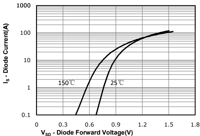
Fig 9: Body-diode Forward Characteristics
