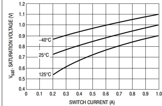
Figure 4. Switch Saturation Voltage
