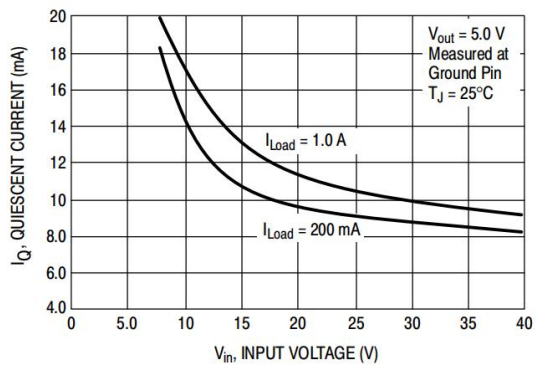
Figure 7. Quiescent Current
