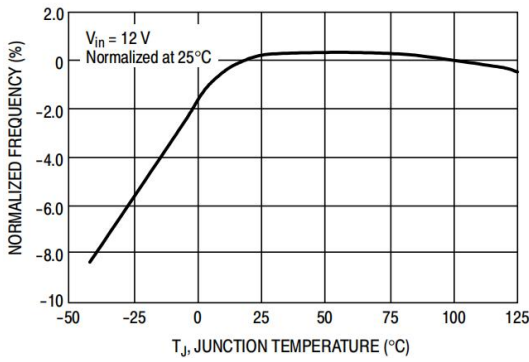
Figure 10. Oscillator Frequency
