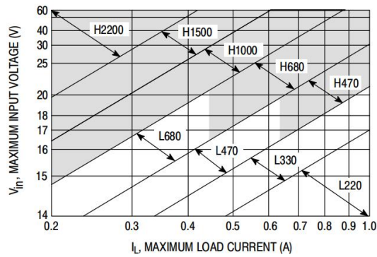
Figure 19. XLM2575-12
