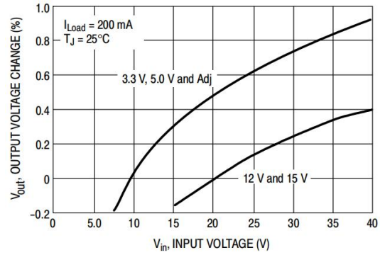
Figure 3. Line Regulation
