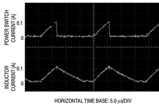
Figure 23. Discontinuous Mode Switching Current Waveforms
