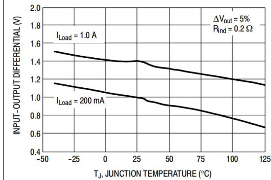
Figure 6. Dropout Voltage
