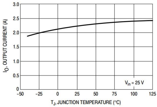
Figure 5. Current Limit
