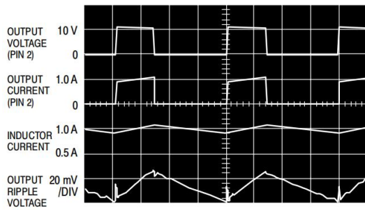
Figure 12. Switching Waveforms
