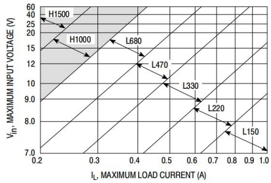
Figure 18. XLM2575-5.0
