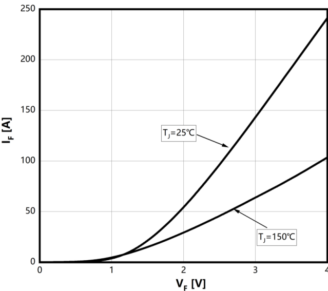
Figure 19. Typical diode forward current as a function of forward voltage
