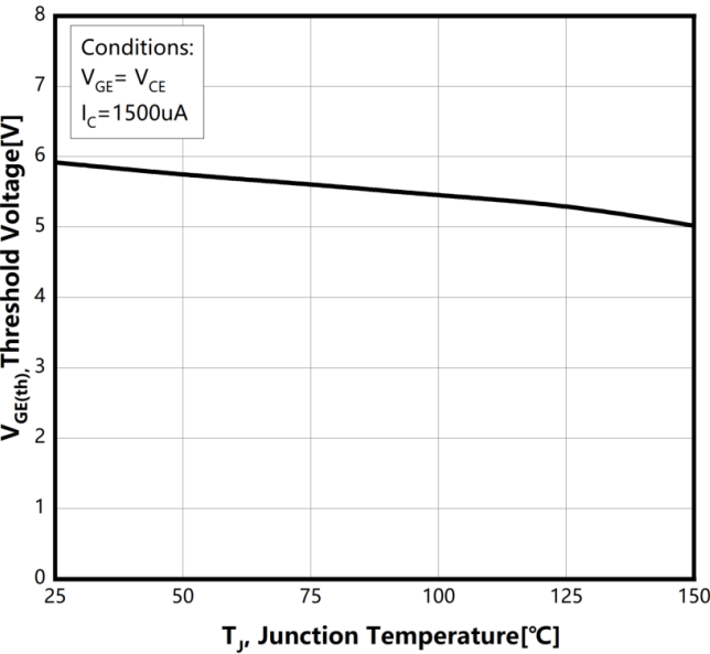
Figure 5. Gate-emitter threshold voltage as a function of junction temperature
