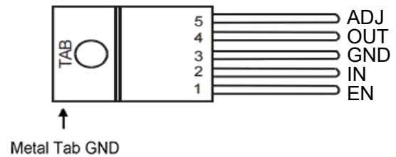
TO-220-5
