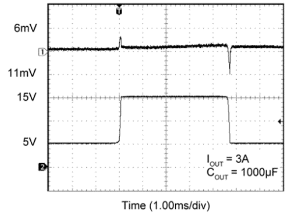
MIC29302AW Line Transient Response with 3A Load, 1000μF Output Capacitance
