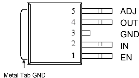
TO-252-4
