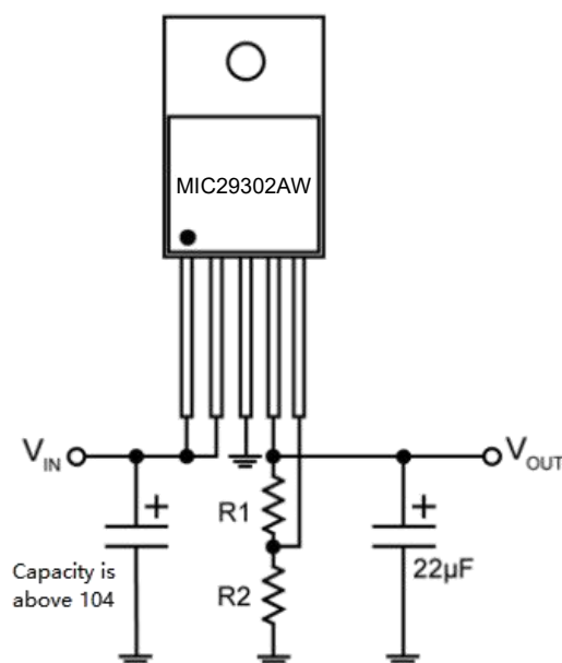
Figure 4. Adjustable Regulator with Resistors
