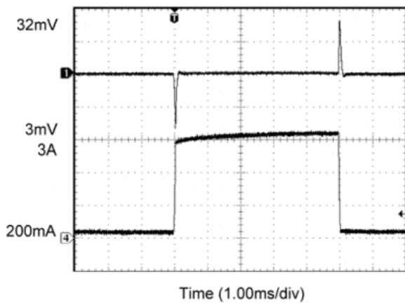
MIC29302AW Load Transient Response
