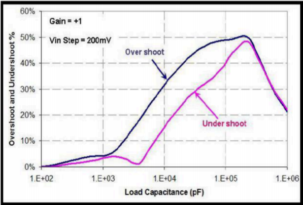
Small-Signal Over-Shoot % vs. C_{\text{LOAD}} , Gain = +1
