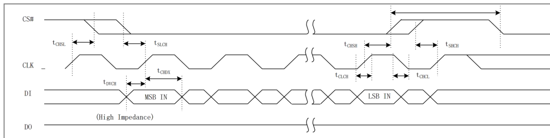
Figure 9.5 Input Timing
