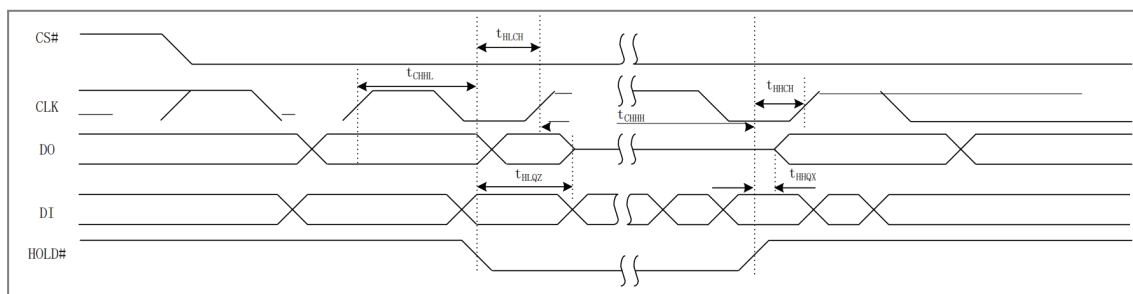
Figure 9.6 Hold Timing
