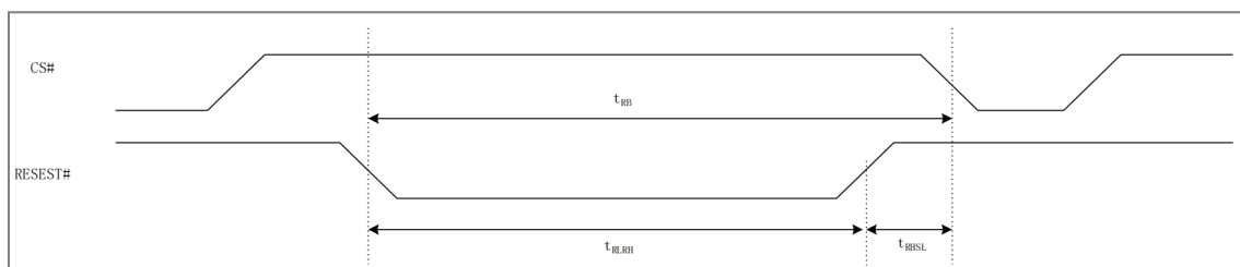
Figure 9.8 Hardware Reset Timing
