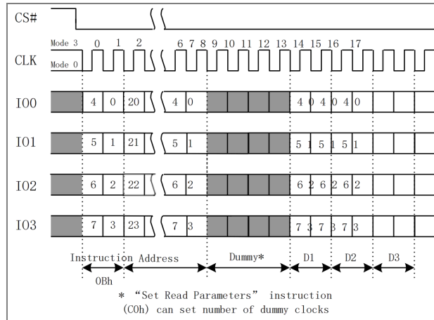
Figure 8.14b Fast Read Instruction (QPI Mode)
