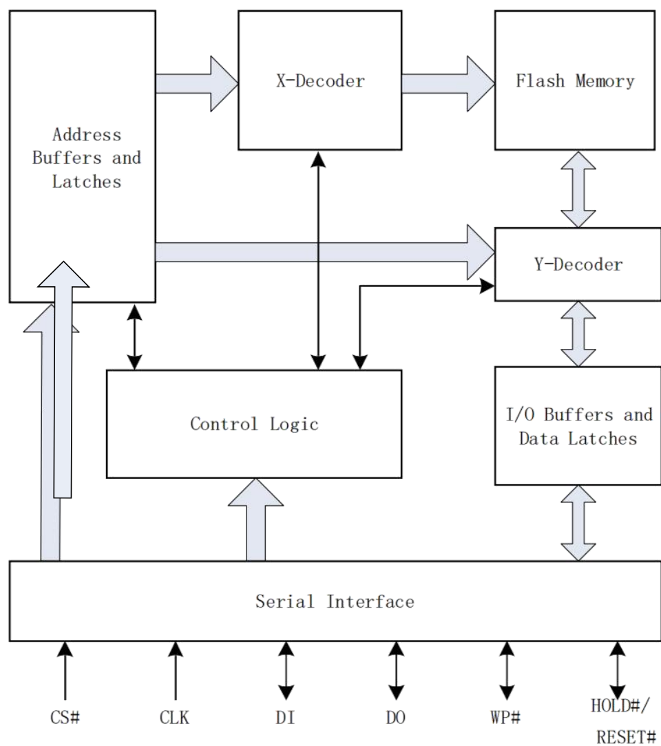
Figure 4.1 Block Diagram
