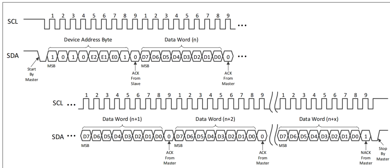
Figure 14 Sequential Read
