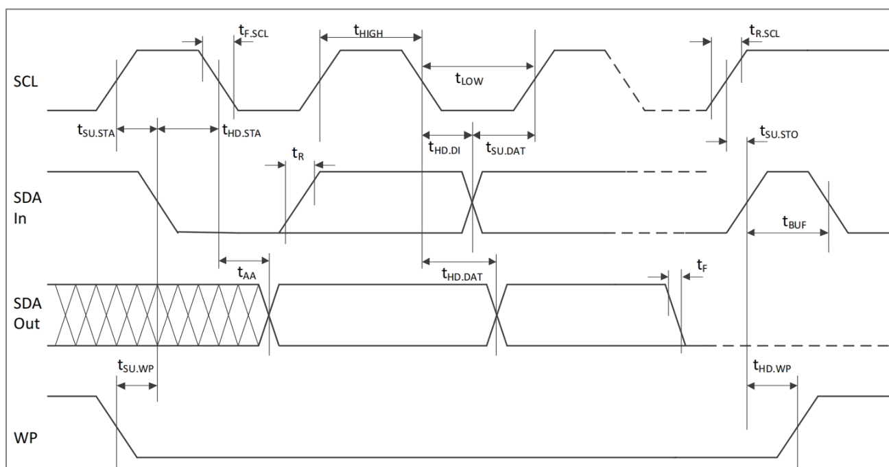
Figure 18 Bus Timing
