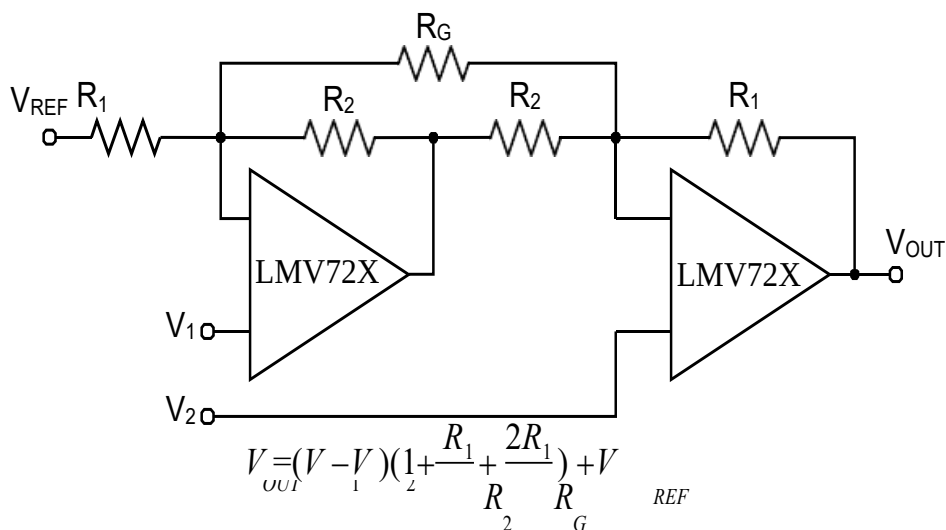
Fig. 17 Instrumentation Amplifier
