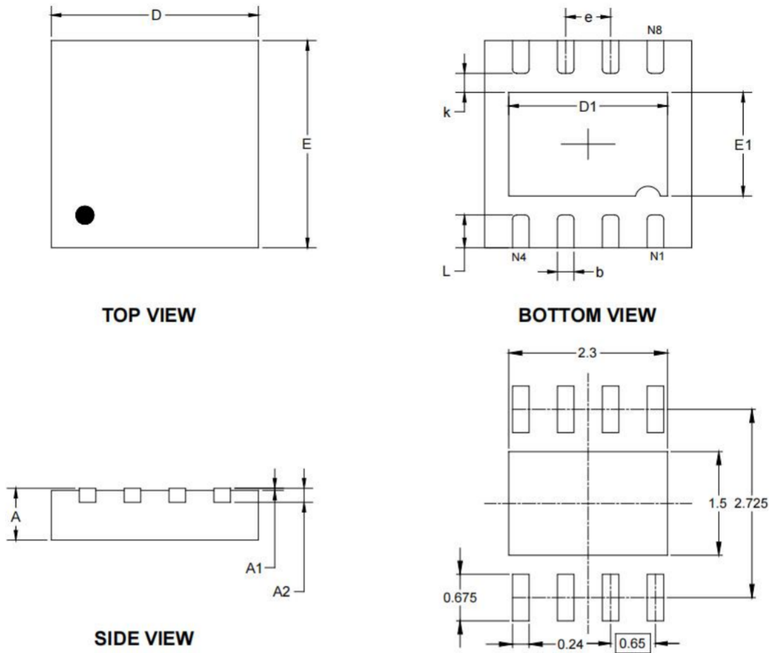
RECOMMENDED LAND PATTERN (Unit: mm)
