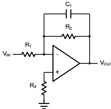
Figure 6. Low Pass Active Filter
