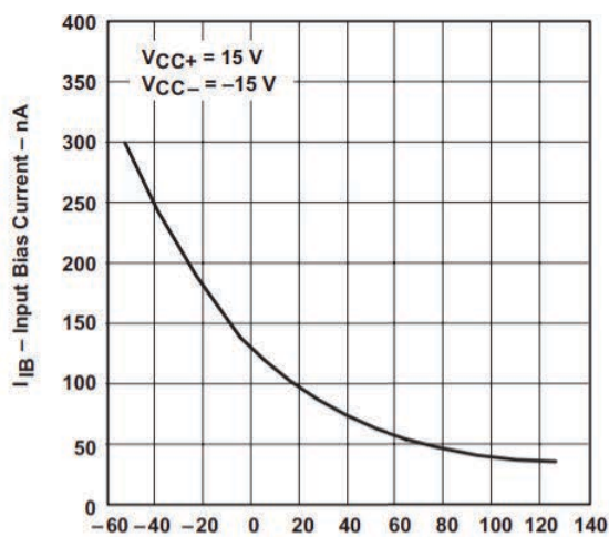
Input Bias Current vs Free-Air Temperature
