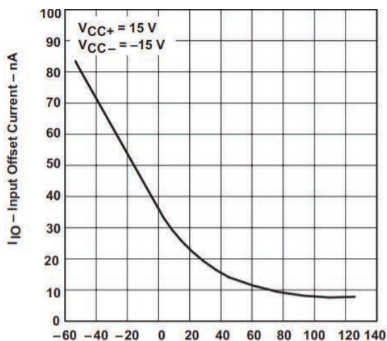
Input Offset Current vs Free-Air Temperature
