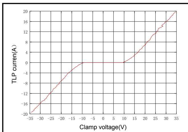
Figure 5: TLP Measurement
