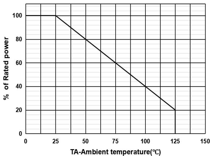
Fig.Power derating vs. Ambient temperature
