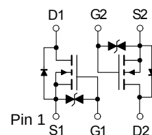
Dual N-Channel MOSFET
