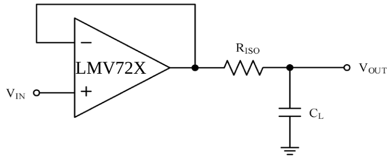
Fig. 14 Indirectly Driving Heavy Capacitive Load
