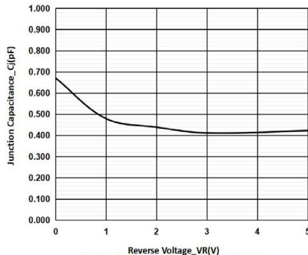
Fig. Junction Capacitance vs Reverse Voltage
