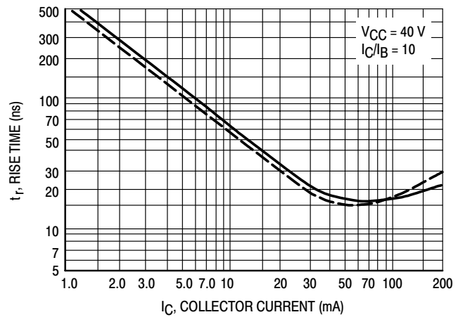
Figure 6. Rise Time
