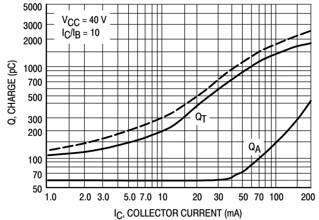
Figure 4. Charge Data
