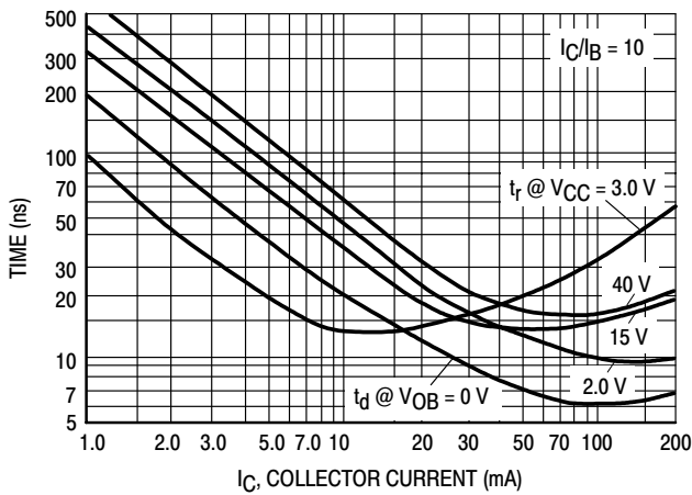
Figure 5. Turn-On Time
