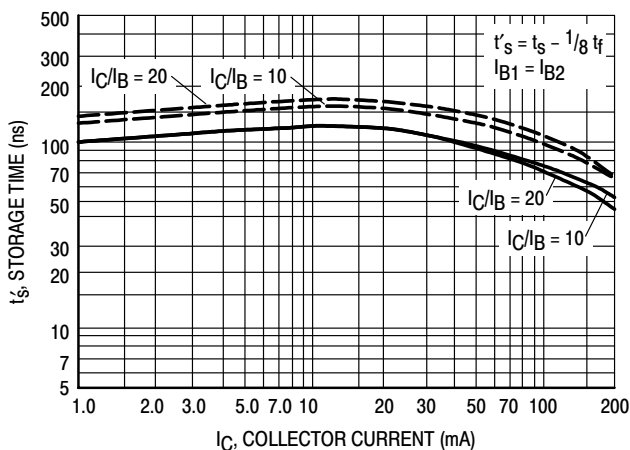
Figure 7. Storage Time
