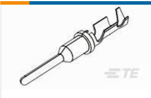
TE Part #1924463-3 PIN, SF, SIZE 16, 18-20 AWG, NI/SN 5/10
