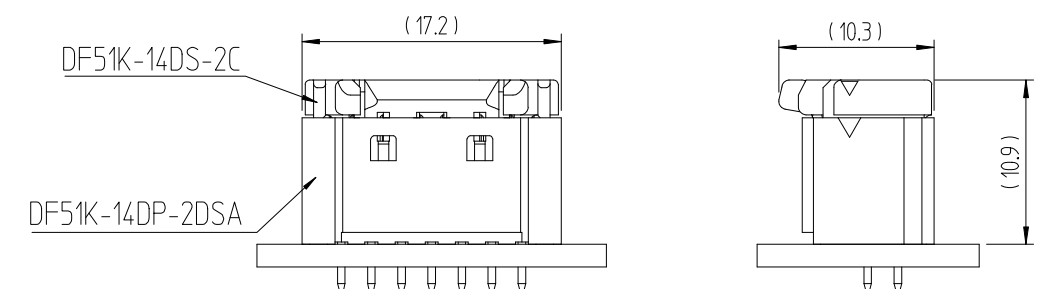
ENGAGEMENT FIGURE (2:1)
