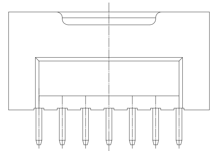
ENGAGEMENT FIGURE (2:1)
