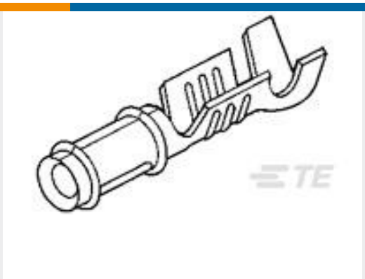
TE Part #350196-1 058 PIN REC 26-20 010TPBECU
