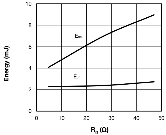
Fig. 9 - Typical Trench IGBT Energy Losses vs. R_g T_J = 125^\circ\text{C} , V_{CC} = 600\text{ V} , I_c = 50\text{ A} , V_{GE} = +15\text{ V}/-15\text{ V} , L = 500\ \mu\text{H}
