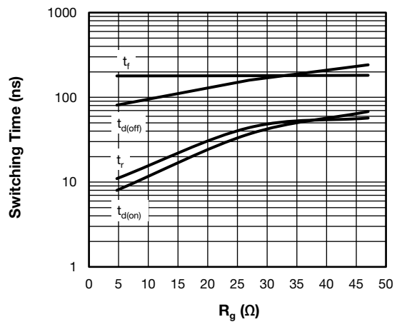
Fig. 10 - Typical Trench IGBT Switching Time vs. R_g T_J = 125^\circ\text{C} , V_{CC} = 600\text{ V} , I_c = 50\text{ A} , V_{GE} = +15\text{ V}/-15\text{ V} , L = 500\ \mu\text{H}
