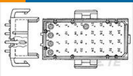
TE Part #640500-5 06P MR HDR ASSY V0
