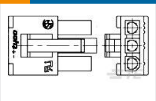
TE Part #1586027-5 5P SR RCPT VAL-U-LOK V0
