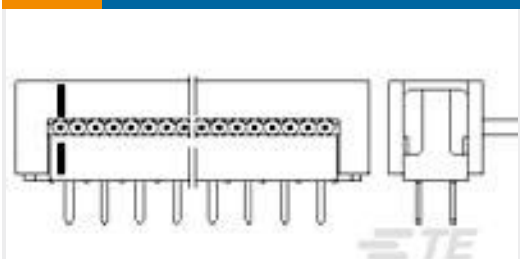
TE Part #1-216093-6 AMP-LATCH PRE-ASSY DIL WITHO
